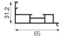
JY-75ZD-31 outframe closing Weight : 0.77 kg/m
