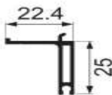
JY-75ZD-29 bottom frame accessories Weight : 0.28 kg/m
