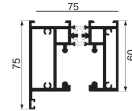
JY75ZD-24 + JY75ZD-25 hanging rail Weight : 1.98 kg/m , 1.59 kg/m
