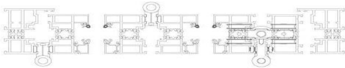
321 folding door assembly drawing .
