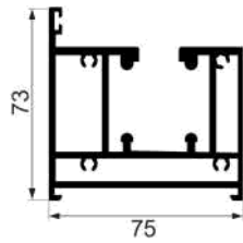
JY-75ZD-28 hanging rail Weight : 3.37 kg/m
