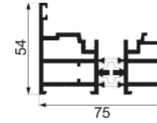
JY75ZD-18 + JY75ZD-19 side frame Weight : 1.5 kg/m , 1.11 kg/m
