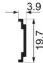
YC-C DG flat aluminum transmission rod Weight : 0.094 kg/m
