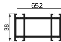
JY-75ZD-26 even-numbered central column Weight : 1.82 kg/m
