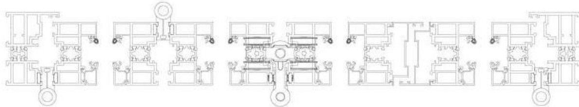
431 folding door assembly drawing:
