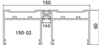
YLF150-A2 Name: Top track thickness: 2.0mm weight: 2.9kg/m
