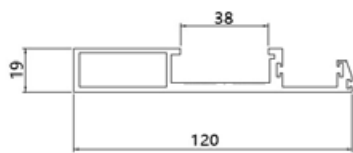
150-05 Name: Vertical interlock frame with handle thickness: 4.0mm weight: 1.64kg/m
