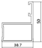
YLF150-23 Name: 4 mm invisible cable thickness: 2.0mm weight: 0.75kg/m
