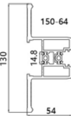
YLF150-C5 Name: Vertical frame with handle thickness: 5.0mm weight: 2.58kg/m
