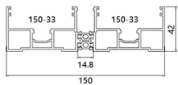
150-XA1 Name: Vertical outer frame thickness: 2.0mm weight: 2.74kg/m
