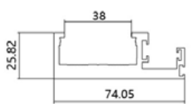
150-59 Name: Vertical interlock frame thickness: 8.0mm weight: 1.91kg/m
