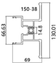
YLF150-C7 Name: Double openable vertical sealing frame thickness: 5.0mm weight: 3.1kg/m
