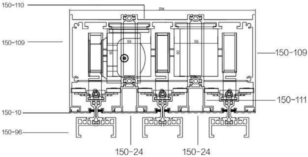
Can be any number of tracks
