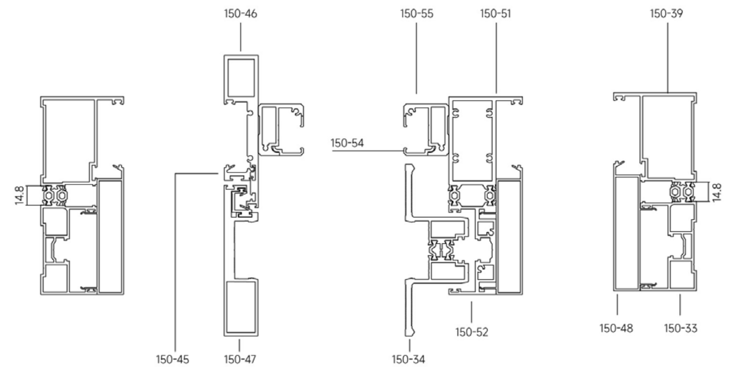
Both sides fixed middle single fan push-pull assembly diagram
