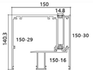
150-A4B Name: Automatic two panels horizontal top track thickness: 4.0mm weight: 6.1kg/m
