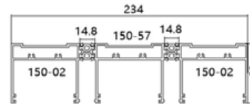
150-SG1 Name: Three panels horizontal top track thickness: 2.0mm weight: 4.57kg/m
