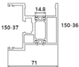
YLF150-C8 Name: 90 degree corner vertical sealing frame thickness: 3.0mm weight: 2.2kg/m
