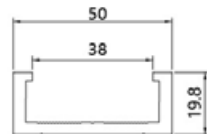
150-06 Name: Vertical frame with fixed glass thickness: 4.0mm weight: 0.83kg/m
