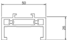
150-90 Name: Horizontal top frame thickness: 3.0mm weight: 1.07kg/m
