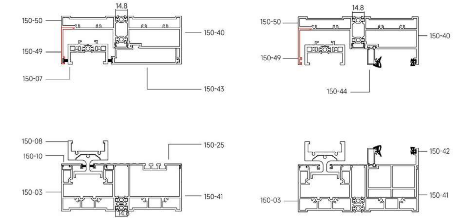
Both sides fixed middle single fan push-pull assembly diagram
