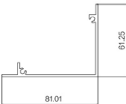
150-21 Name: Sink thickness: 2.0mm weight: 0.84kg/m
