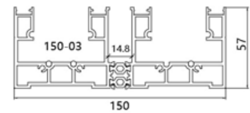
YLF150-A3 Name: Bottom track thickness: 3.0mm weight: 3.8kg/m
