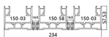
150-SG2 Name: Three panels horizontal bottom track thickness: 3.0mm weight: 6.1kg/m
